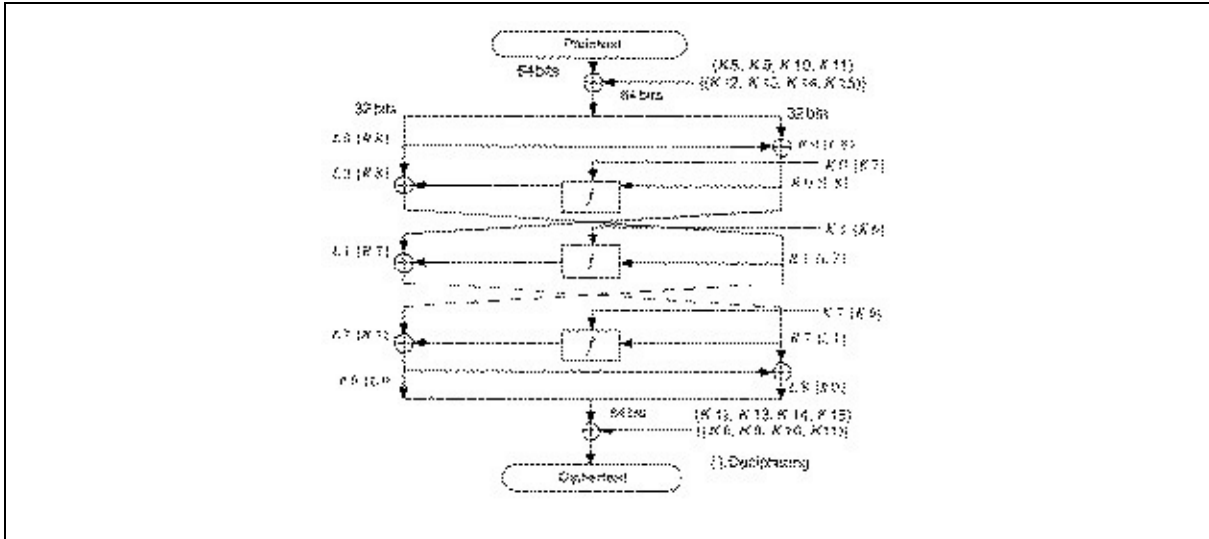
Figure 13.3 One round of FEAL.
