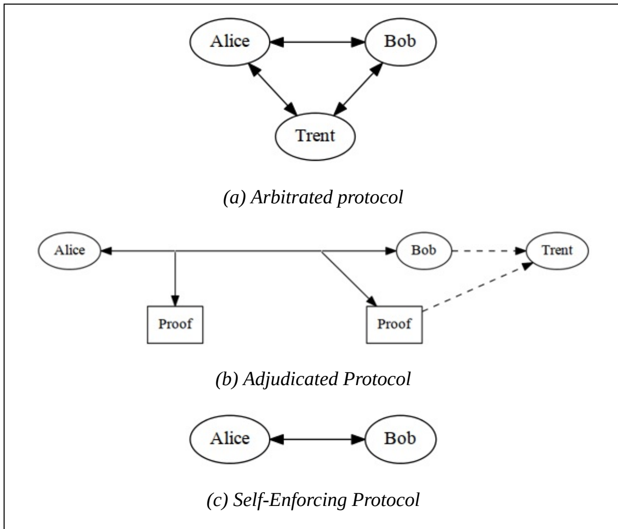
Figure 2.1 Types of protocols.
