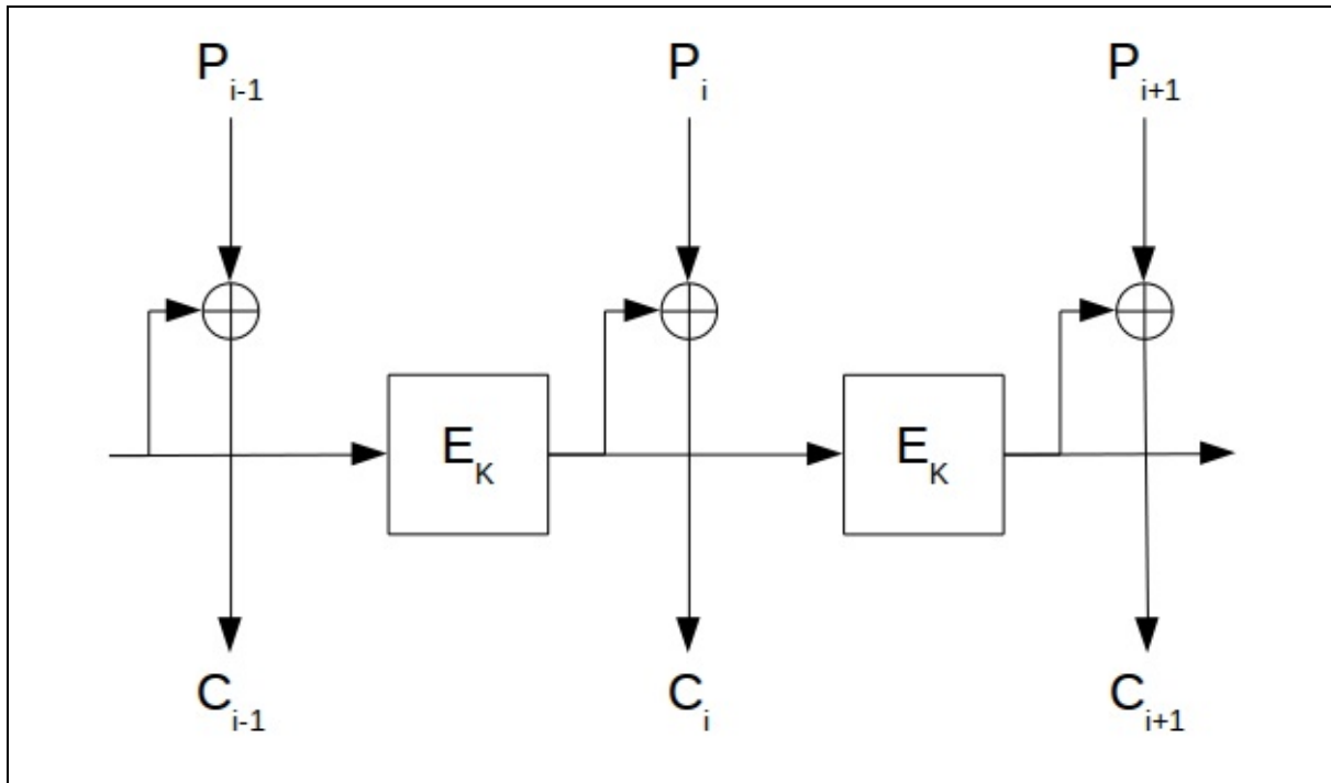
Figure 9.12 n-bit OFB with an n-bit algorithm.
