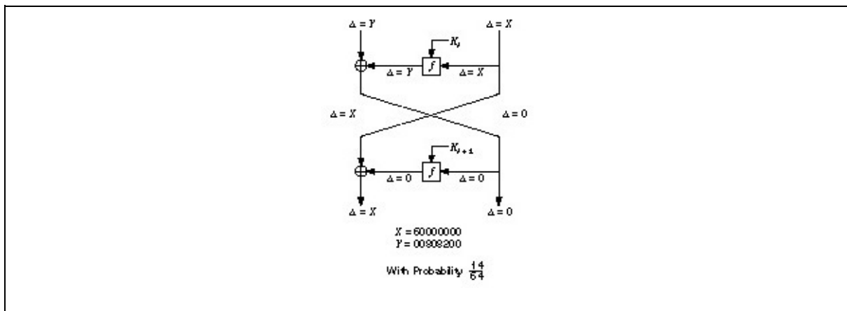
Figure 12.7 A two-round DES characteristic.
