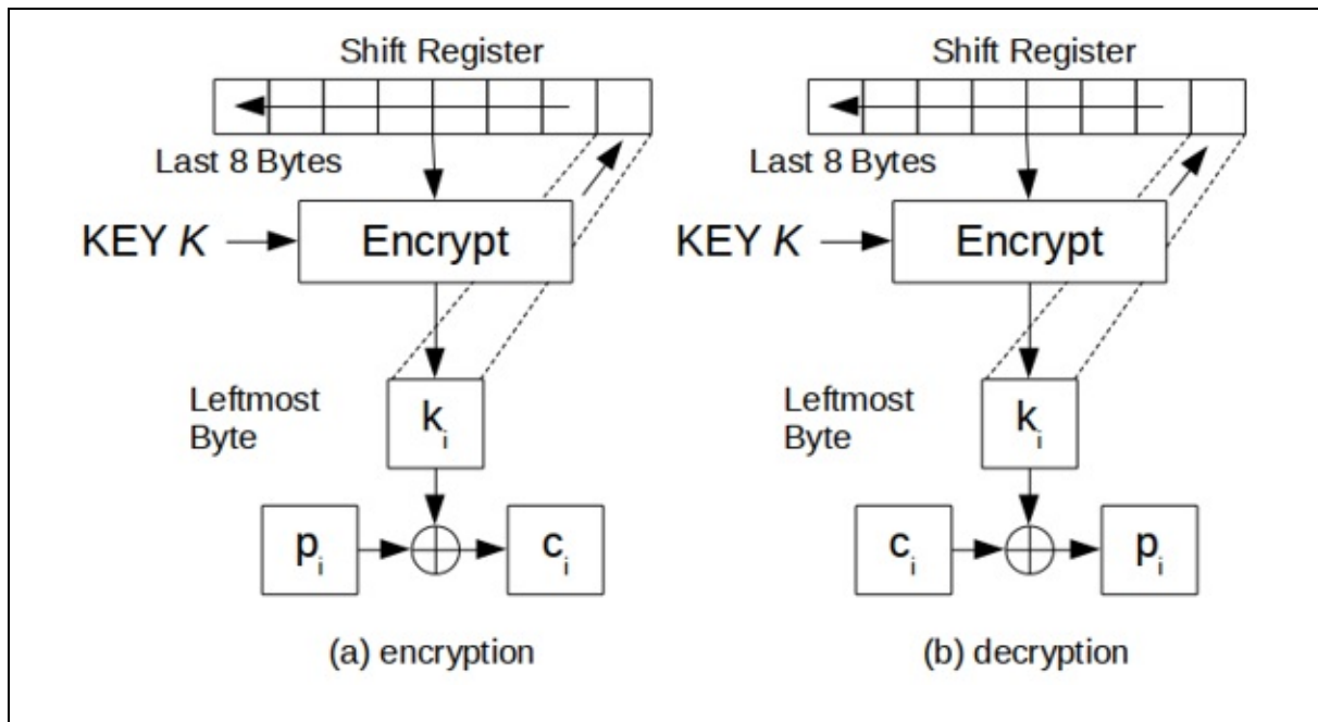
Figure 9.11 8-bit output-feedback mode.
