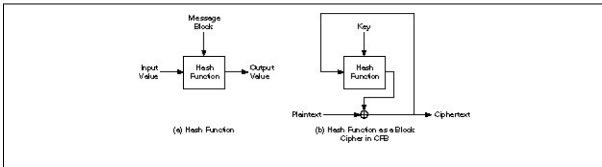
Figure 14.5 Message Digest Cipher (MDC).
