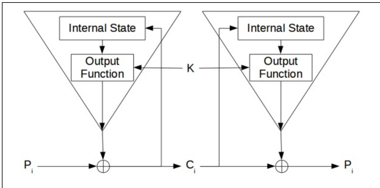
Figure 9.8 A self-synchronizing keystream generator.
