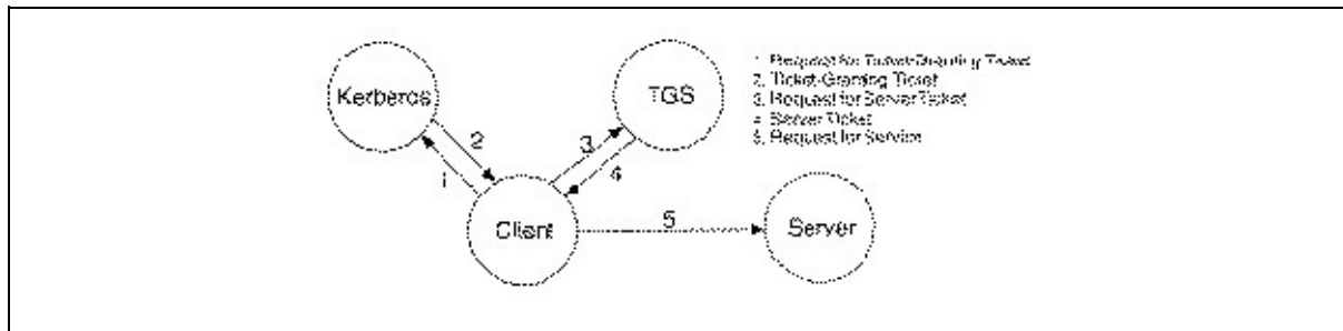
Figure 24.1 Kerberos authentication steps.
