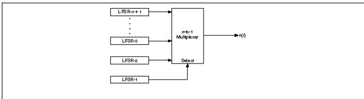
Figure 16.7 Generalized Geffe generator.
