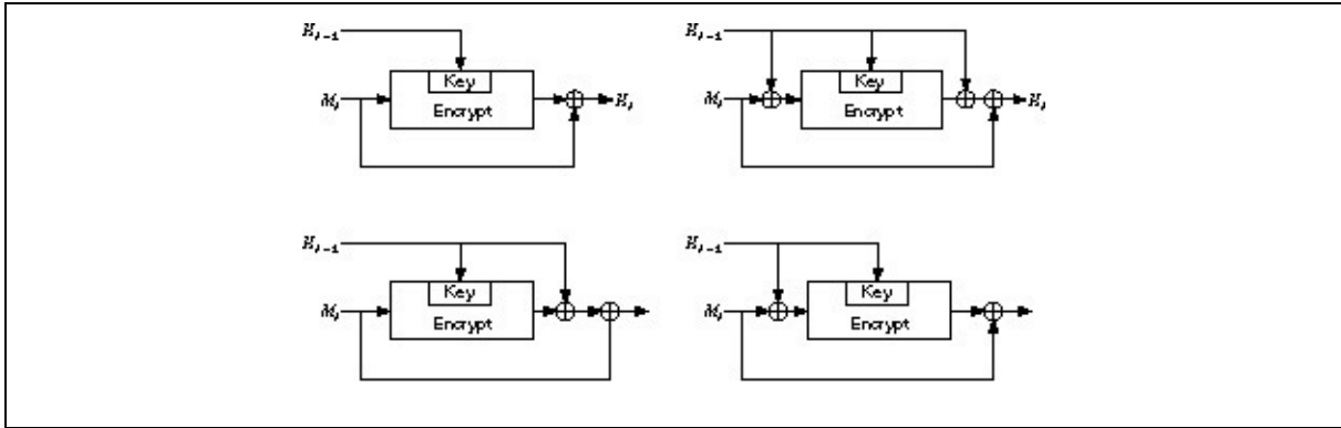
Figure 18.9 The four secure hash functions where the block length equals the hash size.
