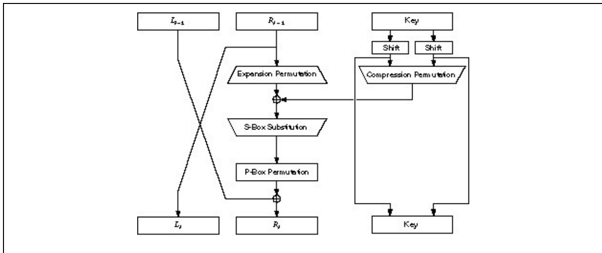
Figure 12.2 One round of DES.
