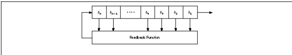
Figure 16.1 Feedback shift register.
