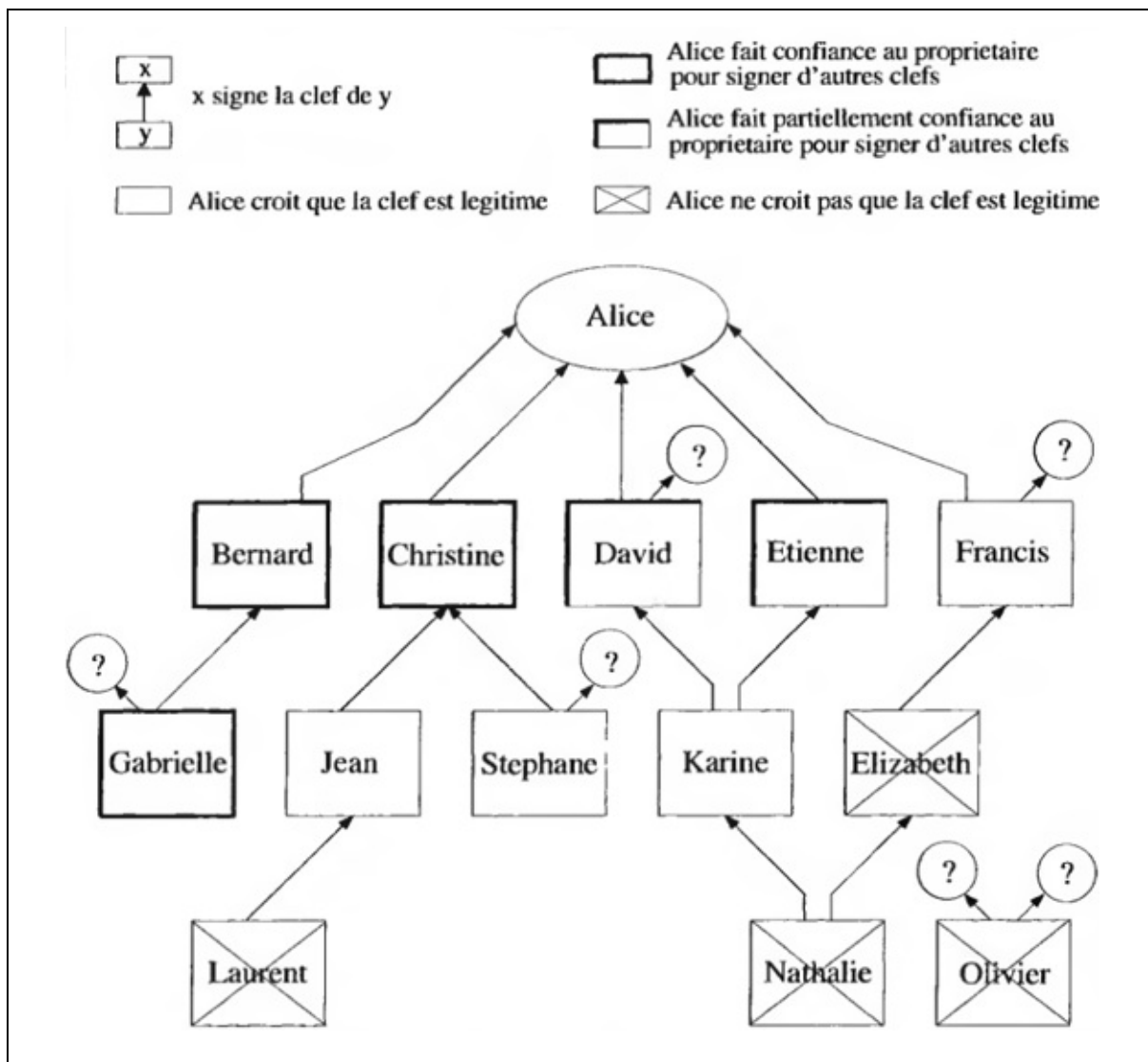
Figure 24.7 PGP trust model.
