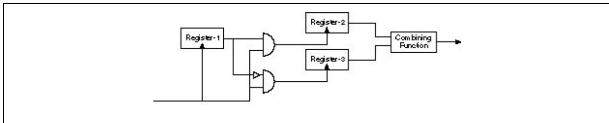
Figure 17.7 Alternating stop-and-go generators.
