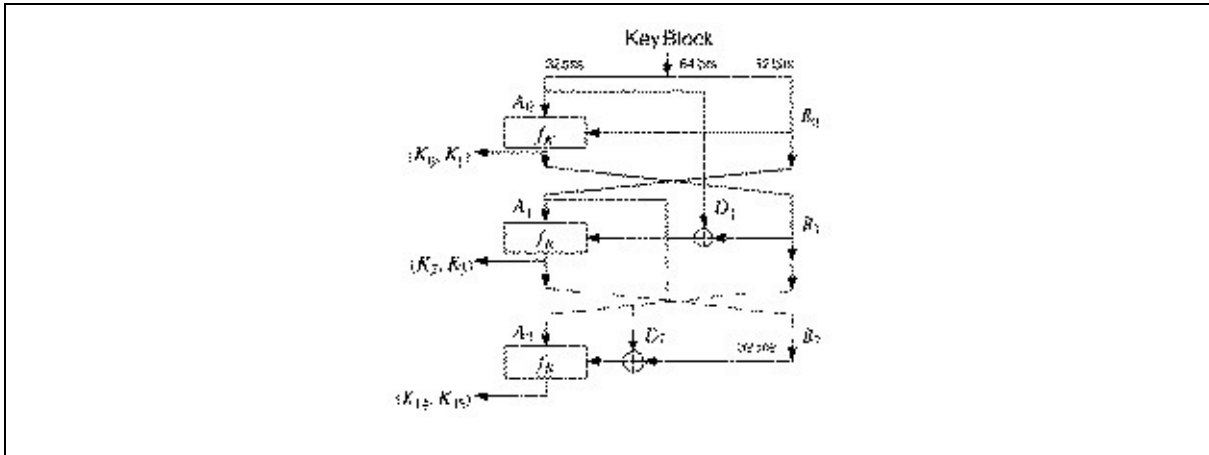
Figure 13.5 Key processing part of FEAL.
