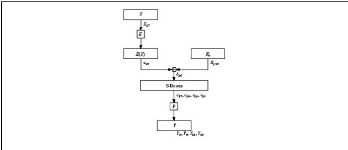
Figure 12.8 A 1-round linear approximation for DES.
