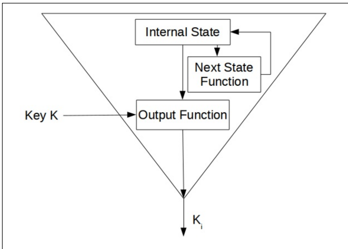
Figure 9.14 A keystream generator in counter mode.
