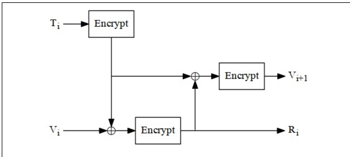
Figure 8.1 ANSI X9.17 key generation.
