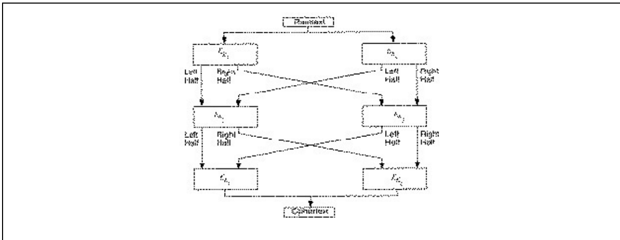
Figure 15.3 Doubling the block length.
