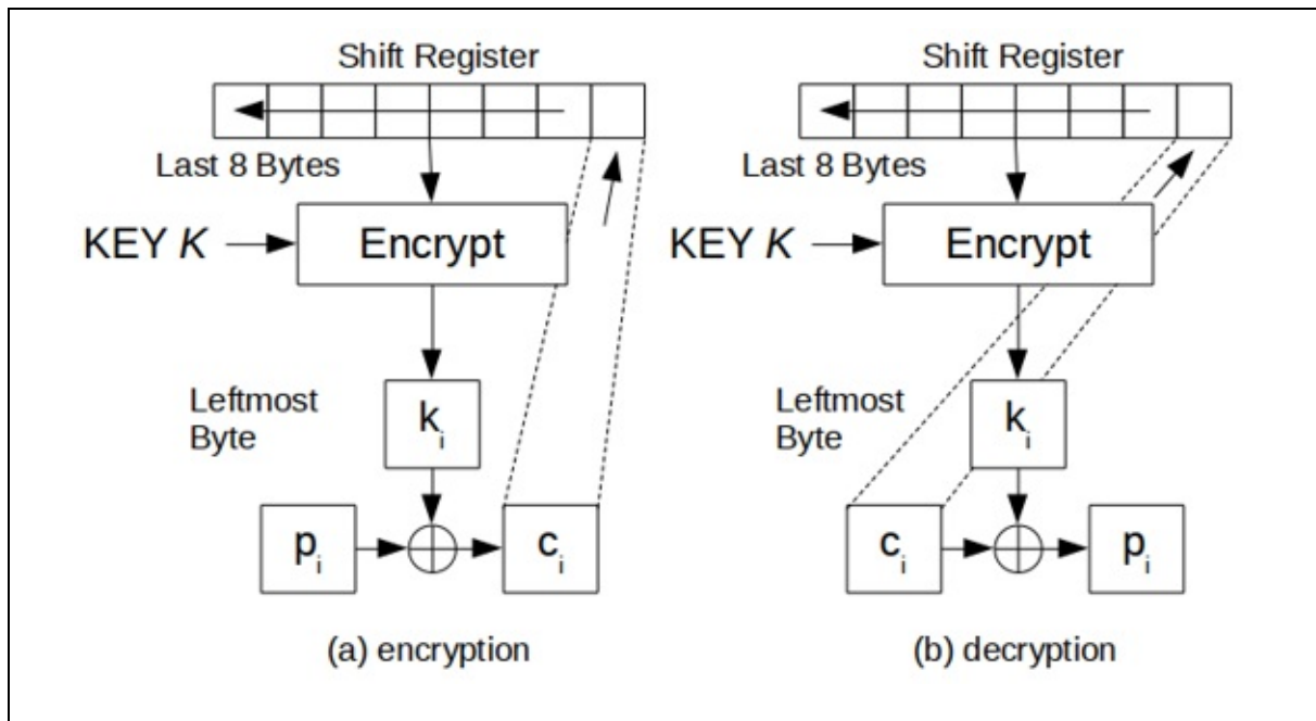
Figure 9.9 8-bit cipher-feedback mode.
