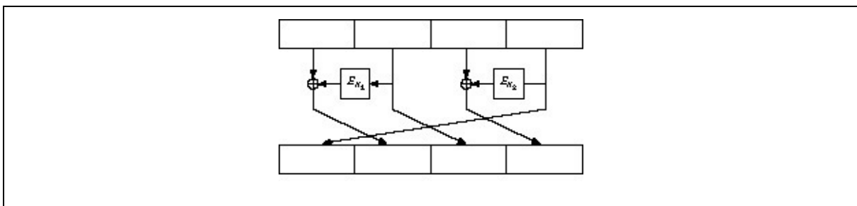
Figure 15.4 One round of \text{xDES}^2 .
