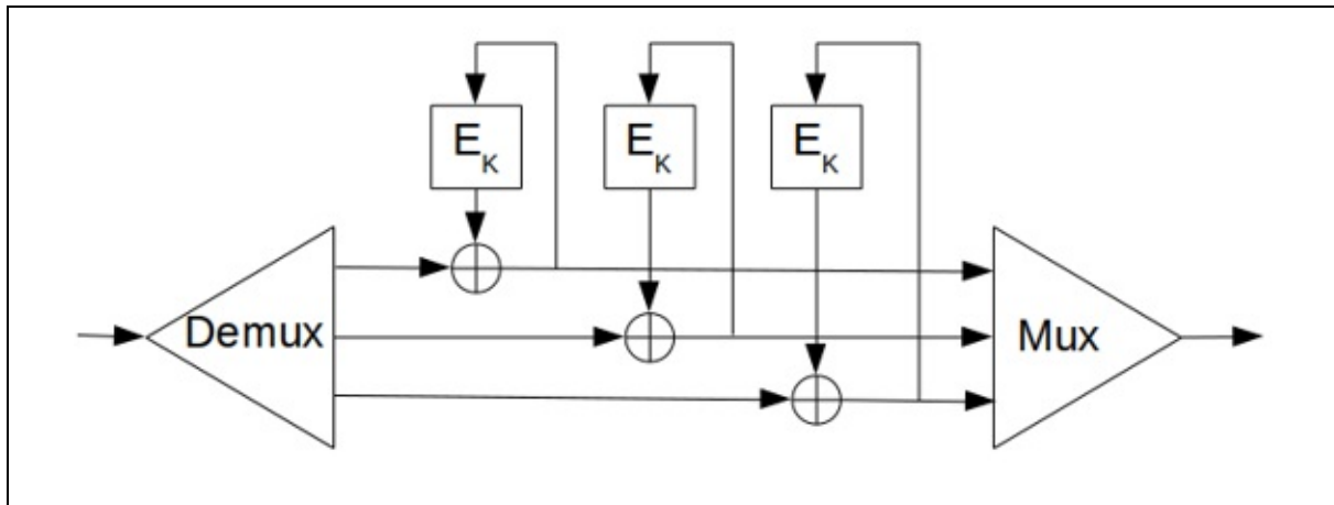
Figure 9.16 Interleaving three CFB encryptions.
