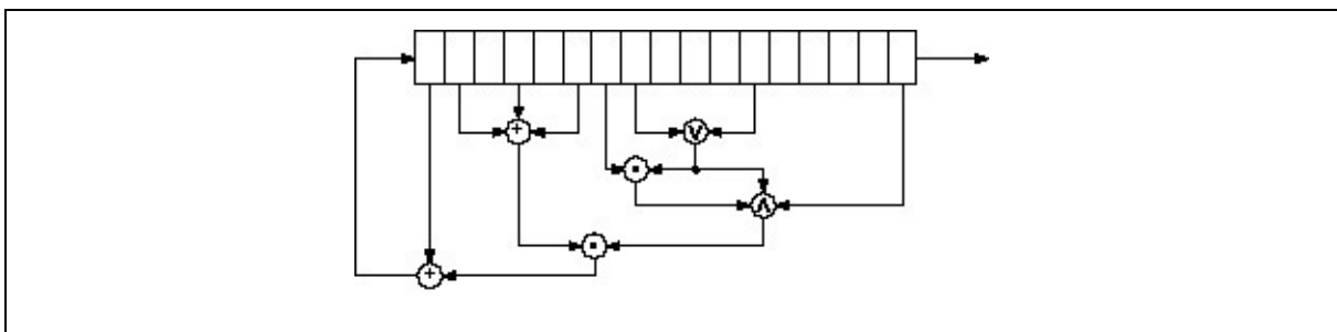
Figure 17.8 A nonlinear-feedback shift register (probably insecure).
