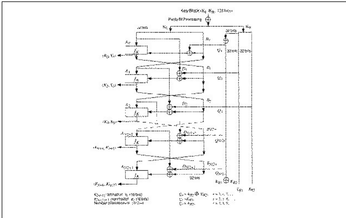
Figure 13.7 FEAL-NX key schedule.
