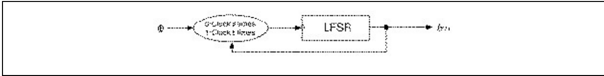
Figure 16.13 Rueppel's self-decimated generator.
