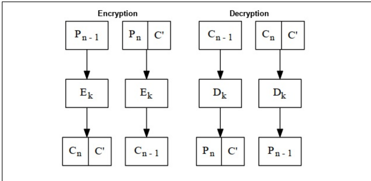
Figure 9.1 Ciphertext stealing in ECB mode.
