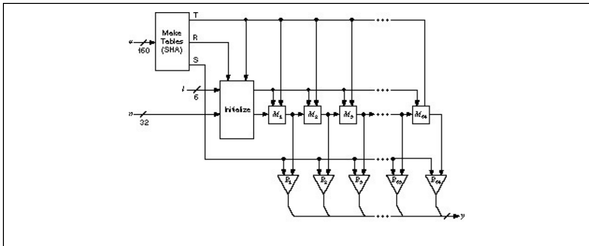
Figure 17.1 The inner loop of SEAL.
