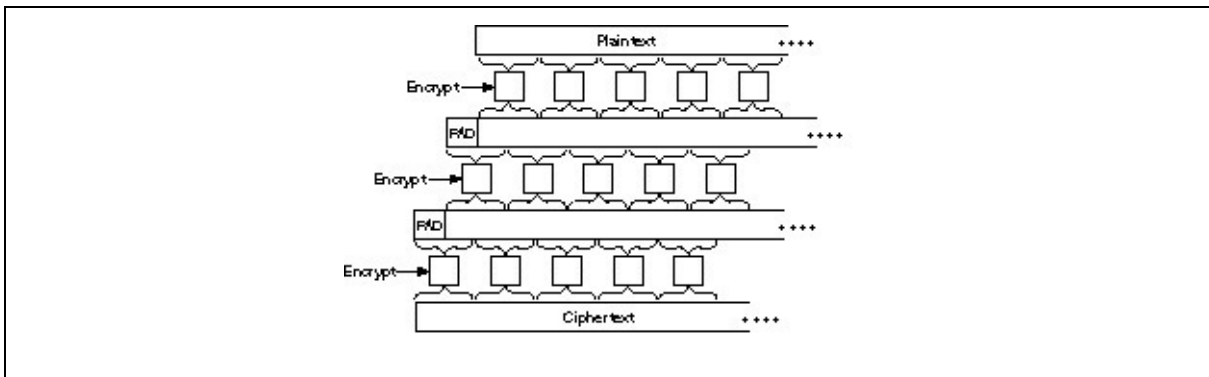
Figure 15.2 Triple encryption with padding.
