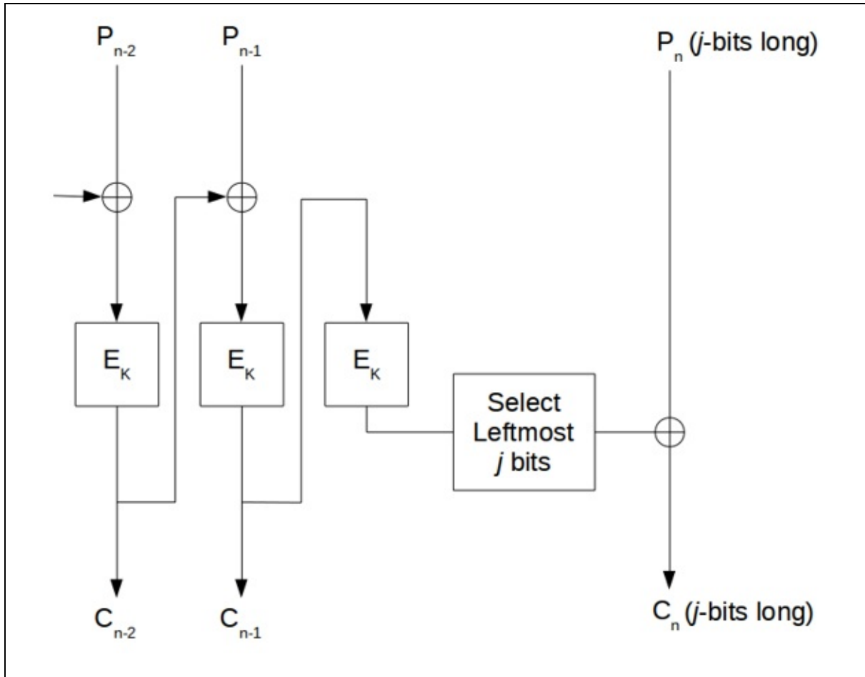
Figure 9.4 Encrypting the last short block in CBC mode.
