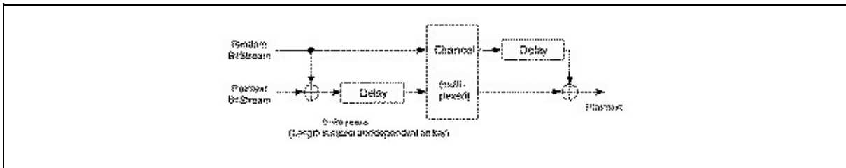
Figure 17.10 Rip van Winkle cipher.
