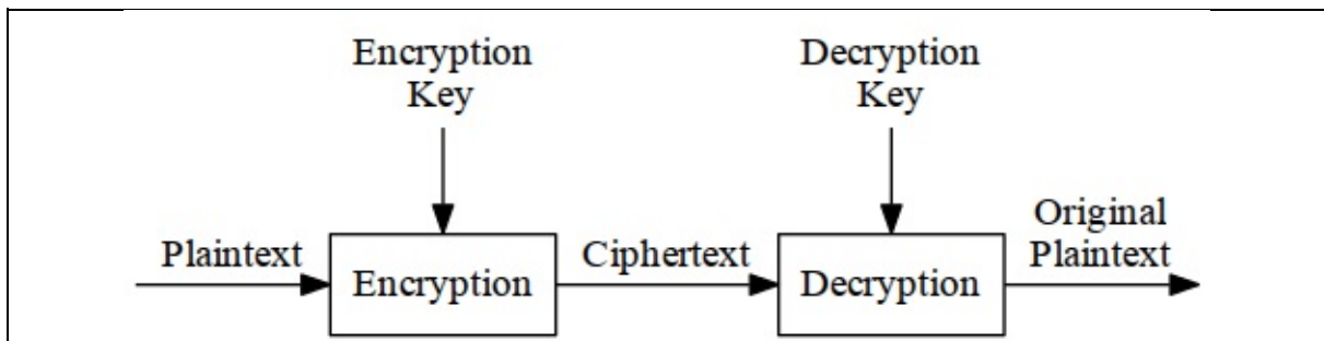
Figure 1.3 Encryption and decryption with two different keys.
