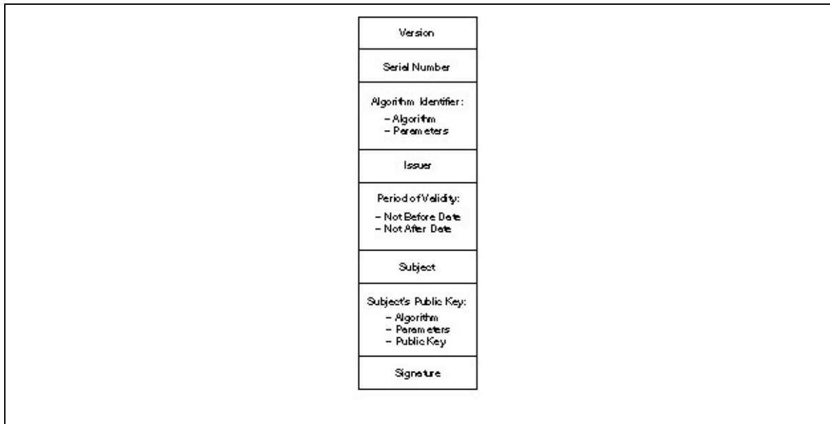
Figure 24.2 An X.509 certificate.
