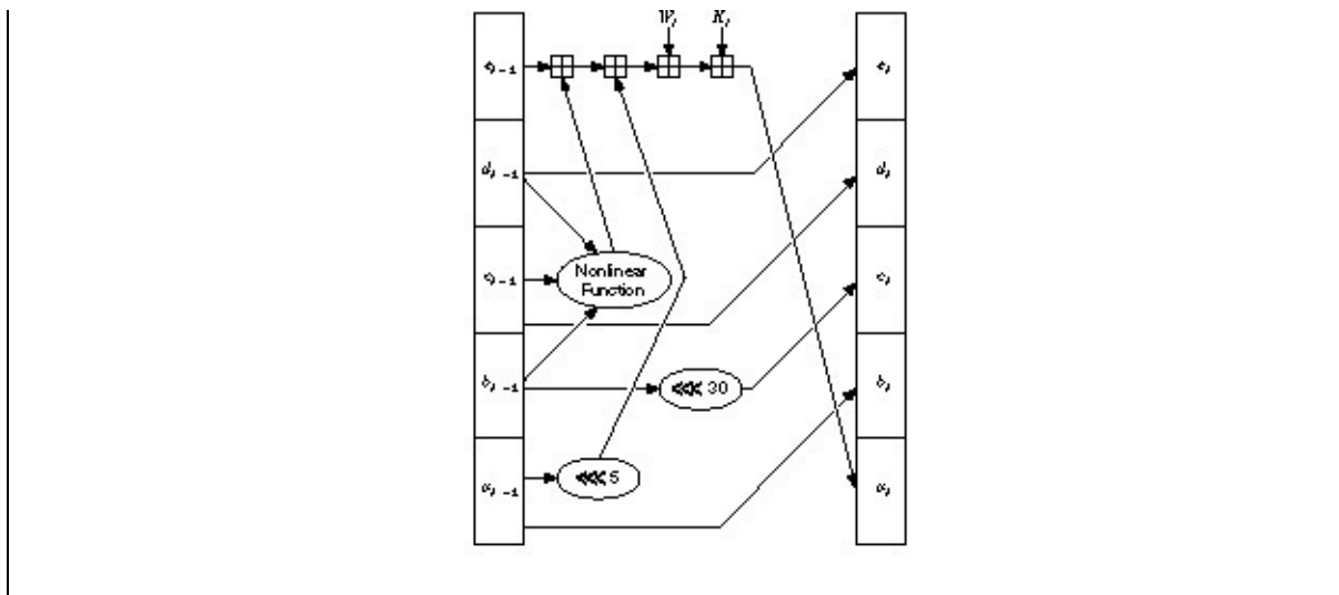
Figure 18.7 One SHA operation.
