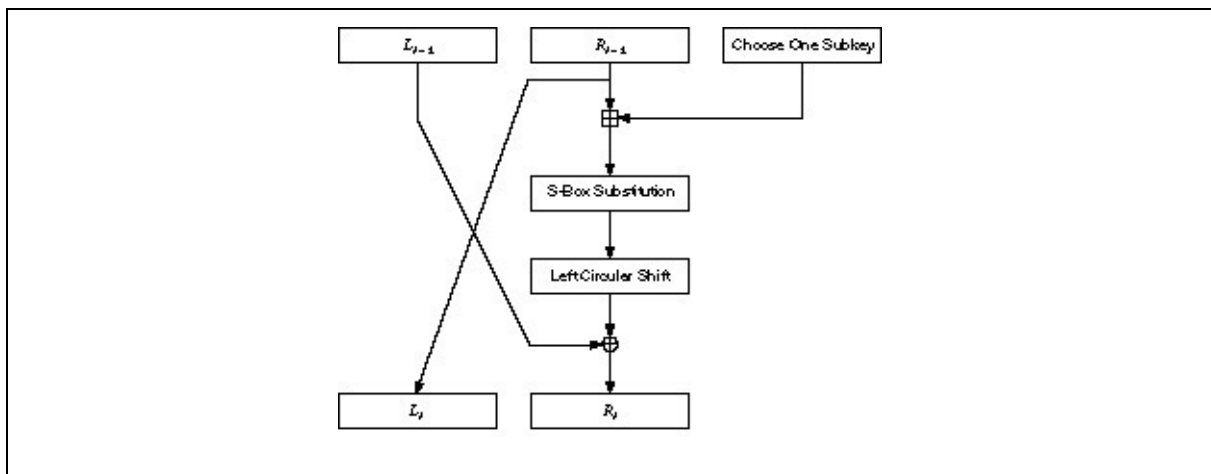
Figure 14.1 One round of GOST.
