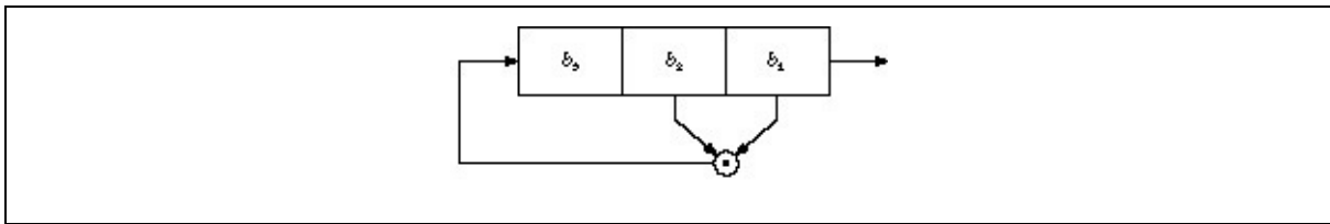
Figure 17.9 3-bit nonlinear feedback shift register.
