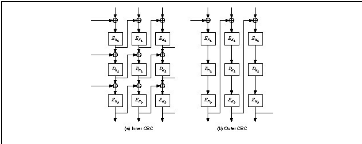
Figure 15.1 Triple encryption in CBC mode.
