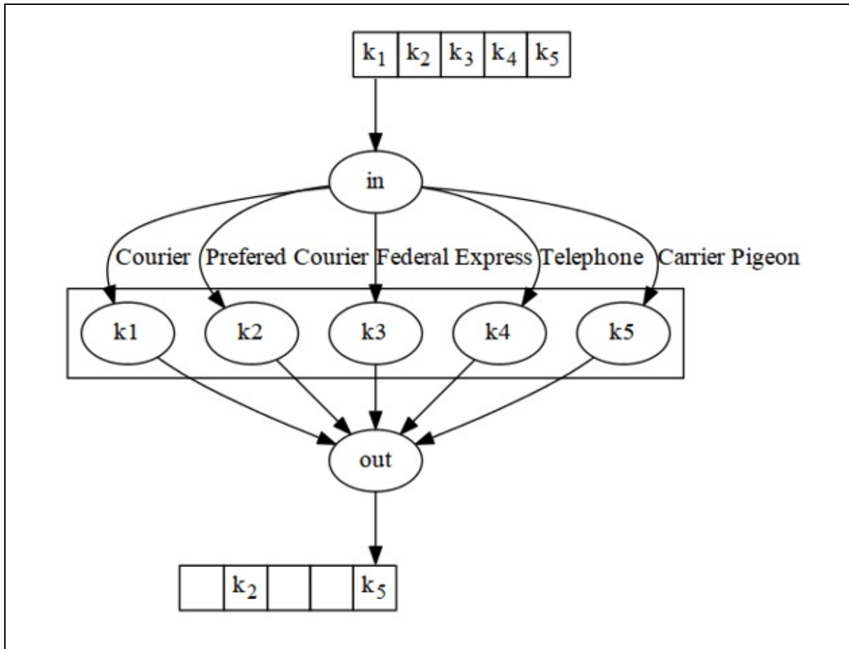
Figure 8.2 Key distribution via parallel channels.
