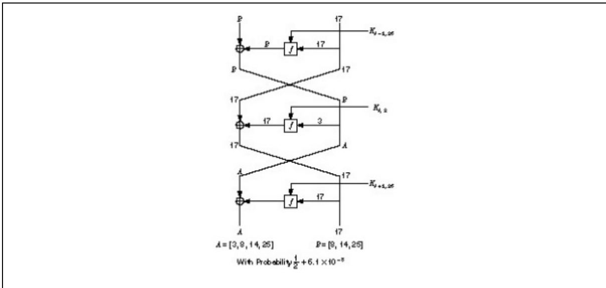
Figure 12.9 A 3-round linear approximation for DES.
