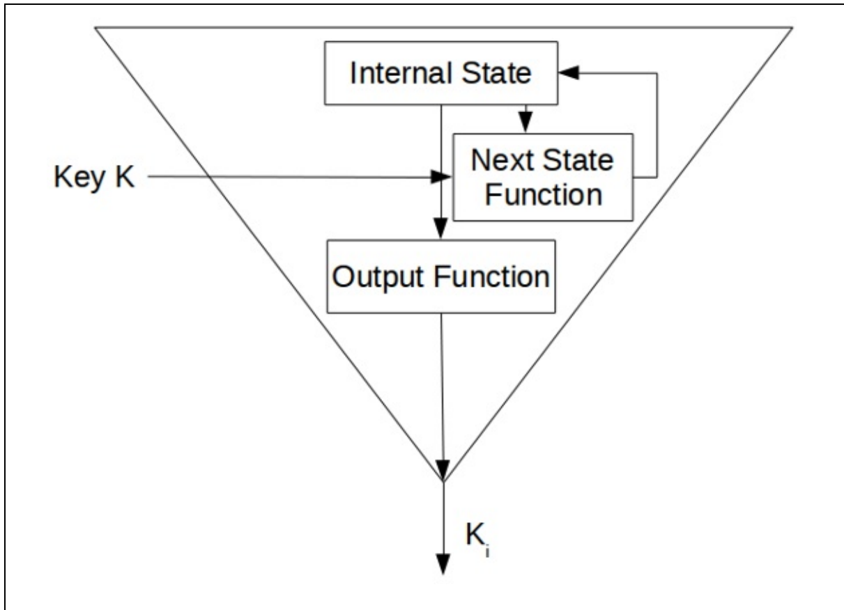
Figure 9.13 A keystream generator in output-feedback mode.
