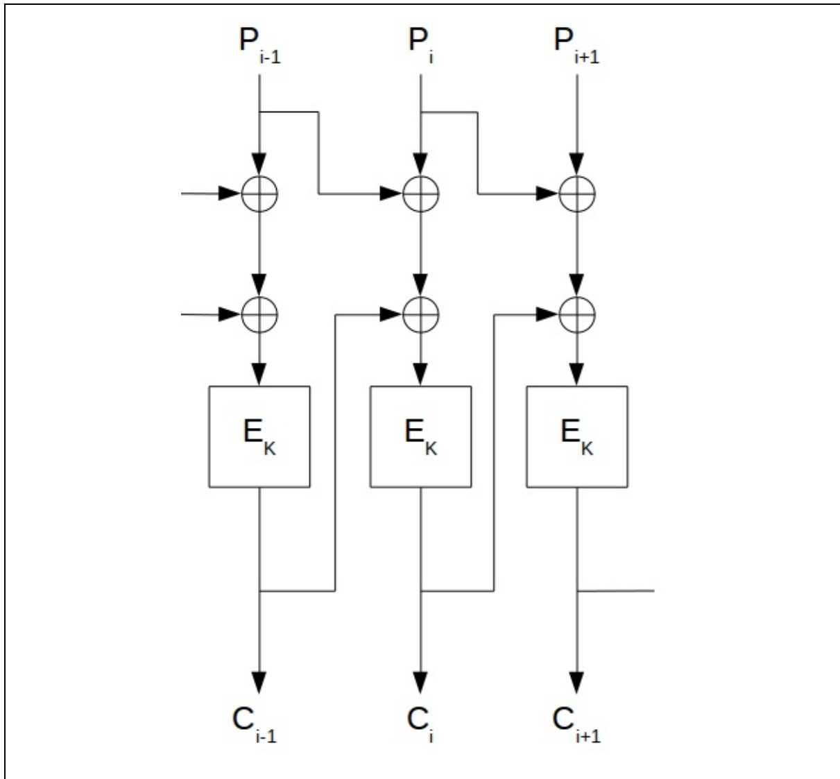
Figure 9.15 Propagating cipher block chaining mode.
