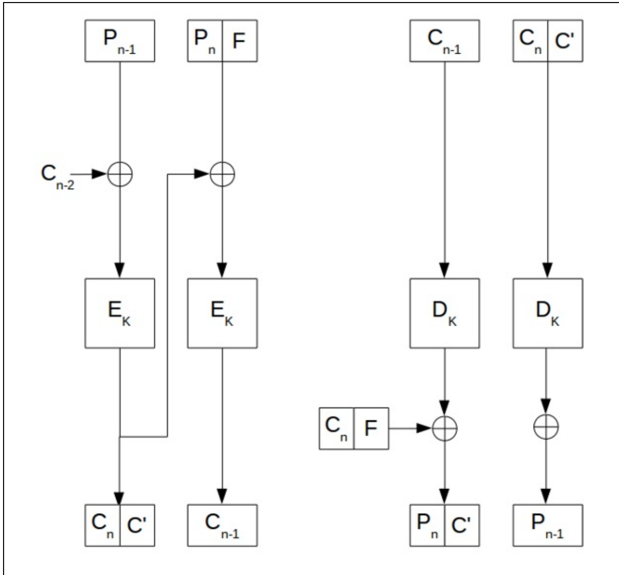
Figure 9.5 Ciphertext stealing in CBC mode.
