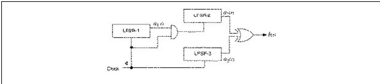
Figure 16.9 Beth-Piper stop-and-go generator.
